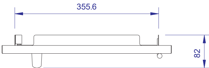
Vertical View
