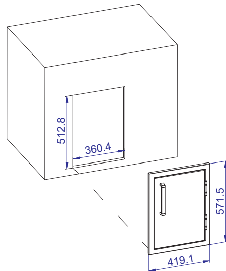
Cutout Size
