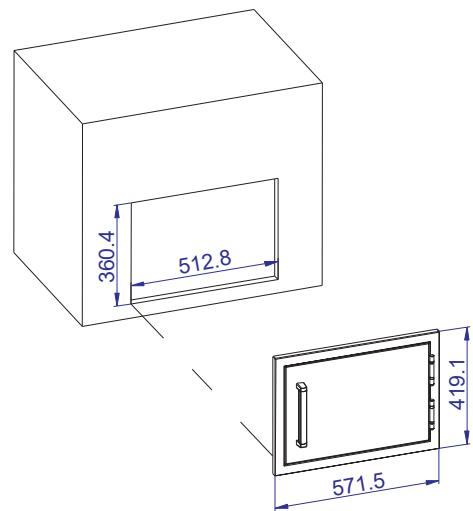
Cutout Size
